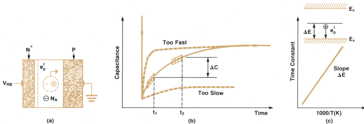
Fig. 2. Principles of capacitance DLTS. (a) Emission of carriers in N + P junction is stimulated by applying bias or infrared radiation. (b) Capacitance transient results when junction is reverse biased. LCR meter measures junction capacitance at two gated time periods. Maximum capacitance change \Delta C occurs at a temperature (i.e., time constant) that is characteristic of the type of defect. (c) Temperature dependence of capacitance time constant.
